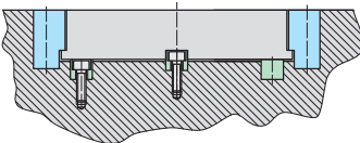
Mounting Example
