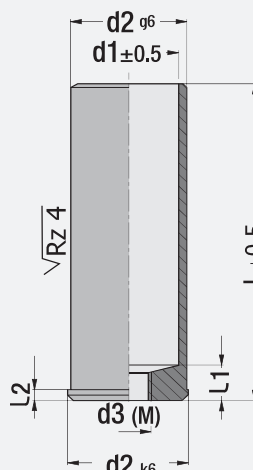
Centring Bush
