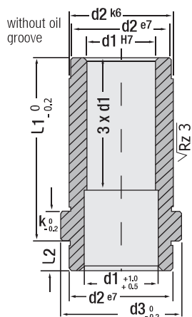
Centring Bush
